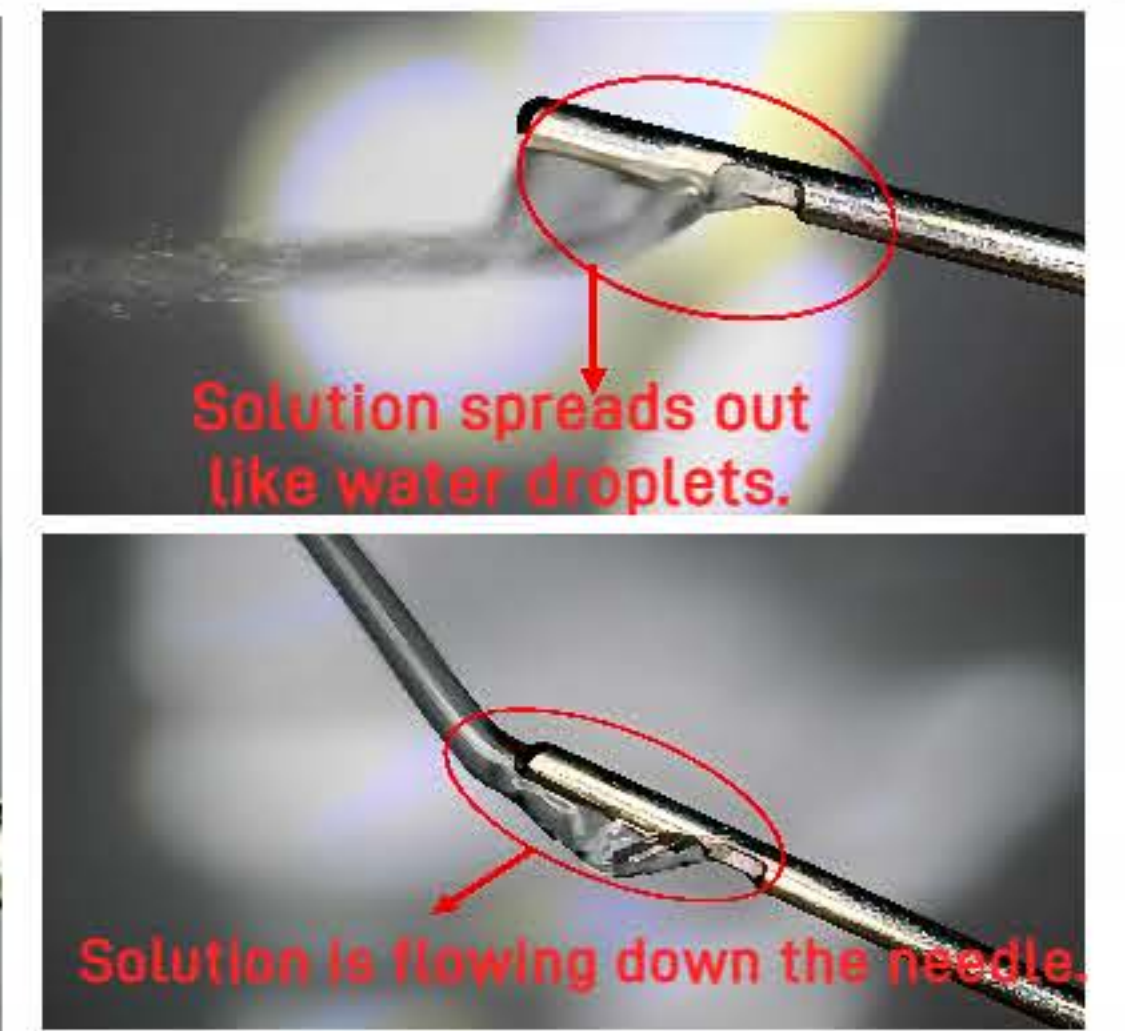
SS Irrigation Needle from other other vendors [2]
