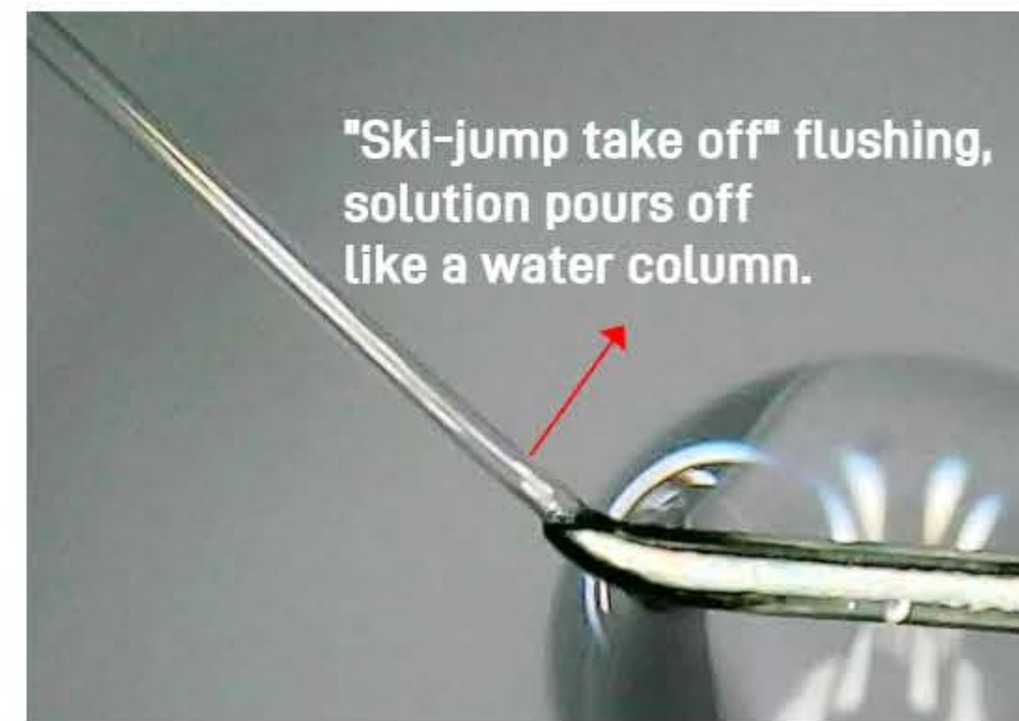
SideIrri Irrigation Needle with sideport spout design, solution pours off like a water column. [1]
