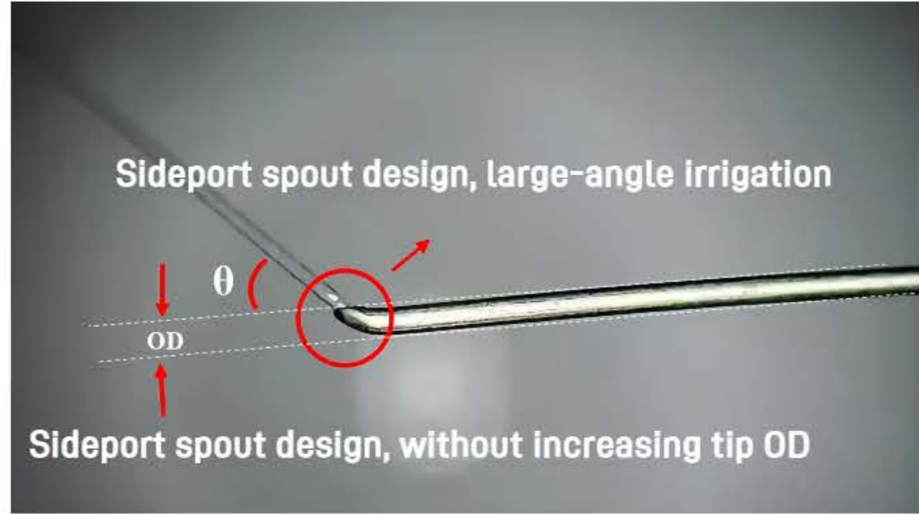
SideIrri Irrigation Needle with sideport spout design, large-angle spray, No cutting on tube wall. [1]
